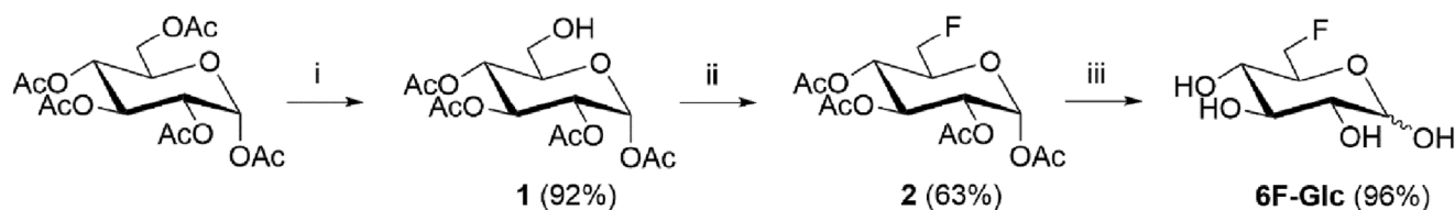
Figure 2. Chemoenzymatic route to the synthesis of 6-deoxy-6-fluoro-glucose (6F-Glc): i) Lipase, phosphate buffer pH 4, dioxane, 24 h at 30 °C; ii) DAST, collidine, DCM; iii) NaOCH 3 , MeOH, Dowex H + .
