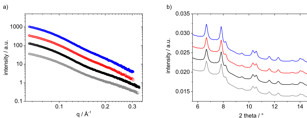
Figure 2. (a) Background-subtracted SAXS scattering data and (b) WAXS diffractograms in an angular range from 5 to 15° 2\theta in the depth close to the electrolyte–catalyst interface: after electrolyte insertion (gray), after catalyst cleaning (black), after 2500 AST cycles (red), and after 5000 AST cycles (blue). The increase in the height and narrowing of the peaks of the diffractogram during the AST protocol imply an increase in particle size, which is in agreement with the mean particle size results. The data in (a and b) are shown with a vertical offset to improve visibility of the different data sets.
