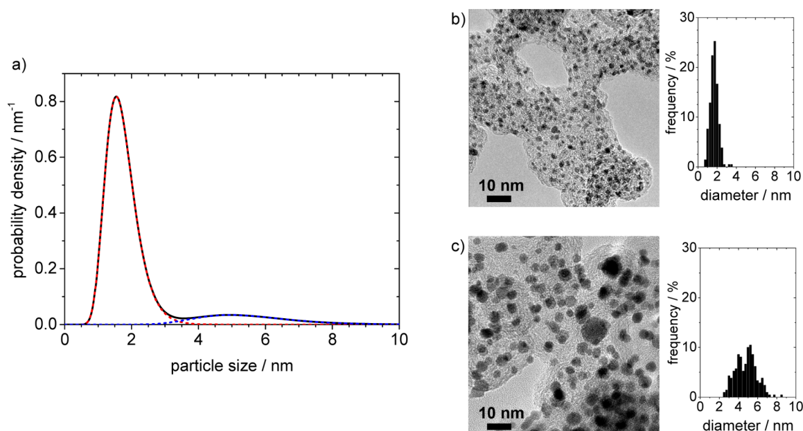
Figure 1. (a) Calculated probability density function of the particle size of the bimodal catalyst after electrolyte insertion (black line) together with the probability densities of the different-size populations (dashed red and blue lines of the small- and large-size population, respectively) in a depth close to the electrolyte–catalyst interface derived from the SAXS data. (b) TEM micrographs and size histograms of the two individual Pt/C catalysts that were mixed to obtain the bimodal Pt/C catalyst.
