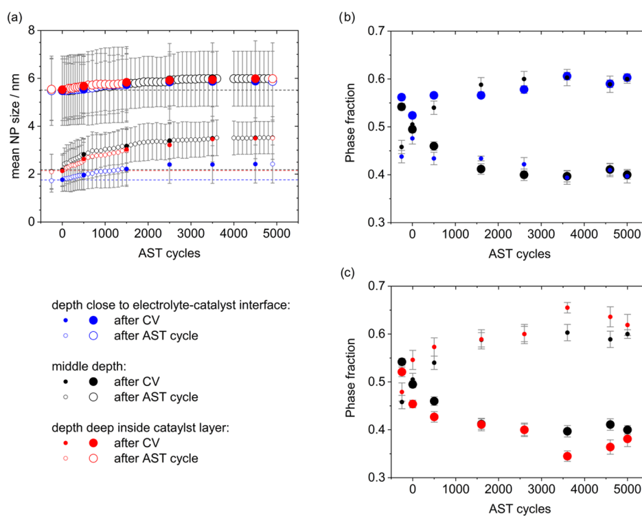
Figure 3. (a) Mean particle size of the bimodal Pt NP/C catalyst (smaller- and larger-size population distinguished with smaller and larger circles) plotted together with the standard deviation of a log-normal distribution applying load cycle conditions as an AST protocol in an operando cell after the AST cycles (empty circles) and after cyclic voltammograms (filled circles) close to the electrolyte (blue), in the middle depth (black), and deeper inside the catalyst layer (red). Phase fractions of the two size populations (small and large circles, for the smaller- and larger-size populations, respectively) obtained from Rietveld refinement measurement of the different depths keeping the particle sizes determined via SAXS constant, (b) close to the electrolyte (blue) and in the middle catalyst layer (black), and (c) in the middle (black, data from Figure 2) and deeper inside the catalyst layer (red) (the red filled circles are placed in front of the red circles and due to an overlap, the black circles are sometimes covered). The data points recorded after electrolyte insertion (before performing the cleaning cyclic voltammograms) are given on the x -axis for a negative AST number.
